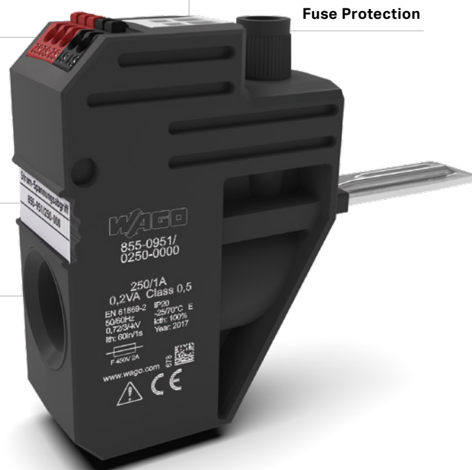
Fuse Protection
